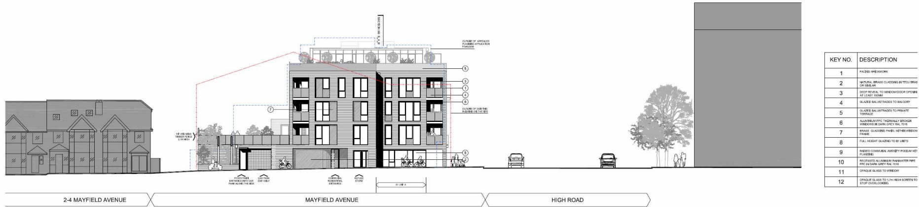
NORTH ELEVATION
